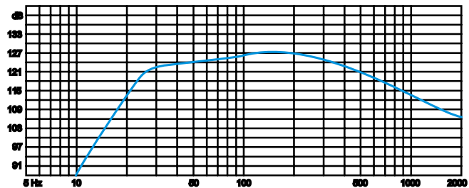
Custom Amplitude Response (dB-SPL/Hz at 1 m) with 500, watts
